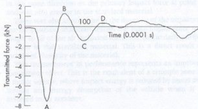
Figure 3 Forces within impacts on standard EVA mouthguard material without air inclusions.
